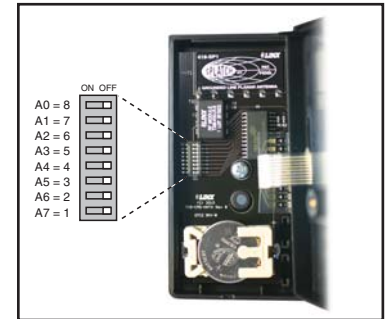
Figure 2: DIP Switch Assignments
