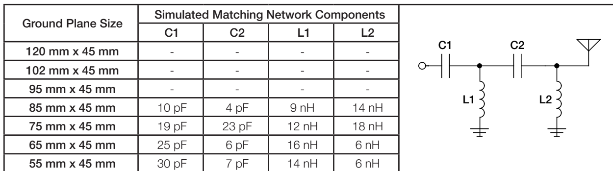
Figure 1. Summary of Ground Plane Sizes and Matching Networks Presented
