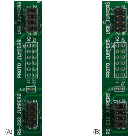
Figure 6: 250 Series Development Board Jumpers; (A) for USB Interface; (B) for RS-232 Interface
