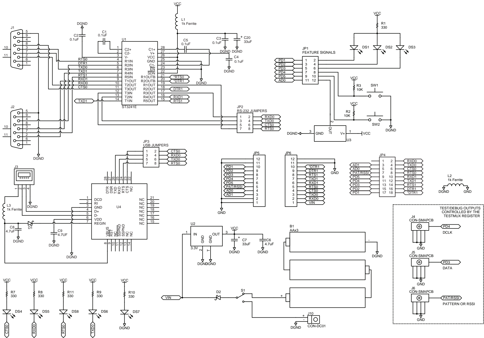
Figure 21: 250 Series Master Development Board Schematic
