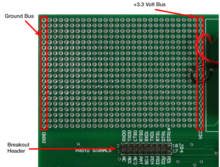
Figure 14: The Development Board Prototyping Area
